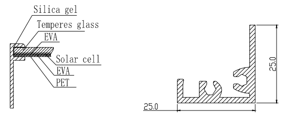
A-A' section Section B-B' SCALE 10:1
