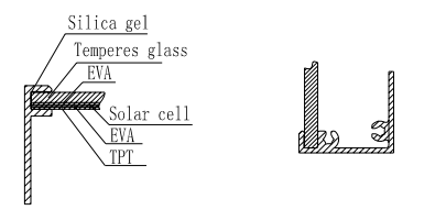
A-A' section B-B' section Scale 10:1
